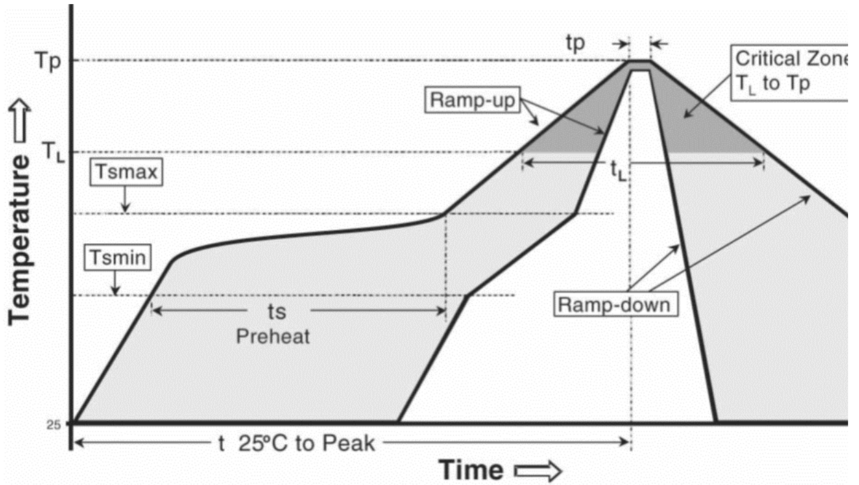
Figure 7 – Temperature profile.
