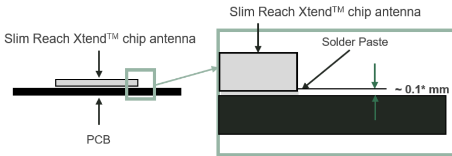
Figure 6 – Soldering Details.
