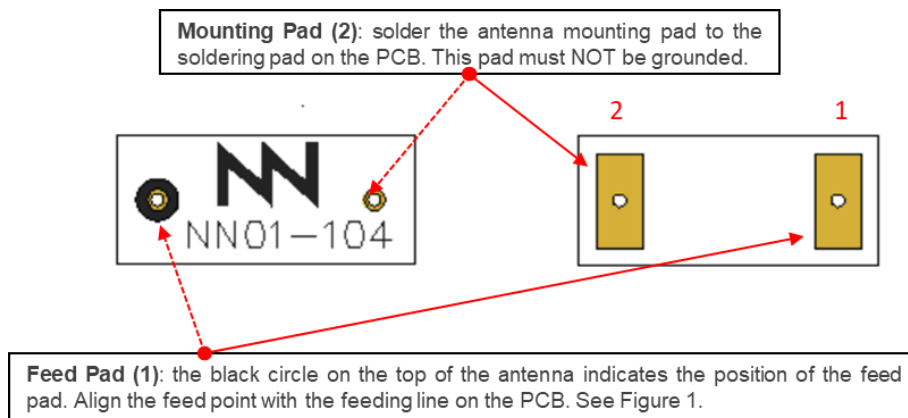
Figure 5 – Pads of the Slim Reach Xtend™ chip antenna.
