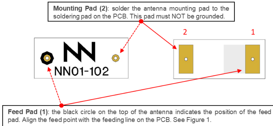
Figure 5 – Pads of the Compact Reach Xtend™ chip antenna.
