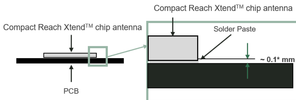
Figure 6 – Soldering Details.
