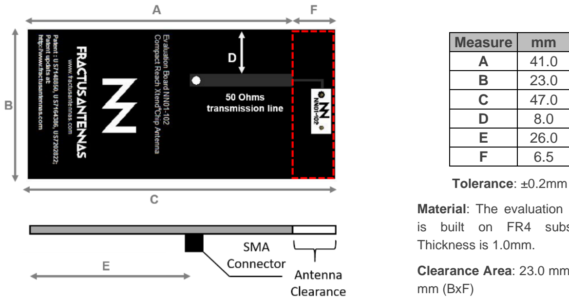
Figure 1 – EB_NN01-102. Compact Reach Xtend™ Evaluation Board.
