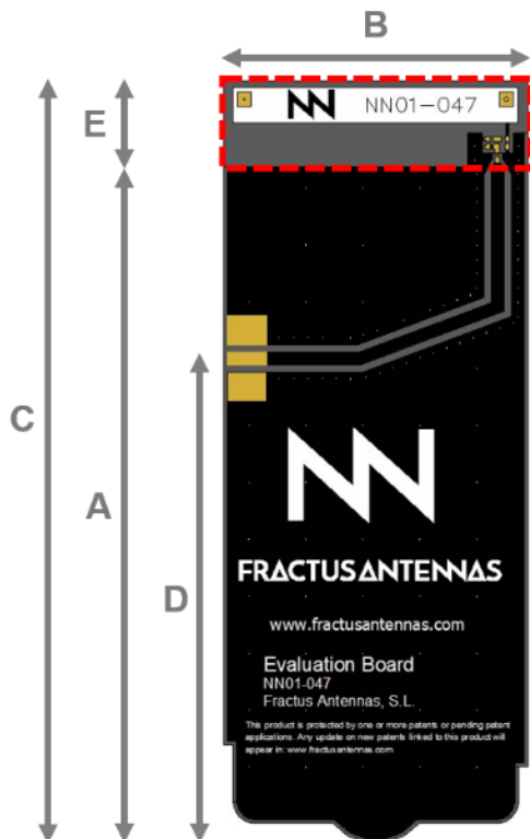
Figure 1 – EB_NN01-047. TVNow™ Dual Band (UHF+Lband) DVB-H.
