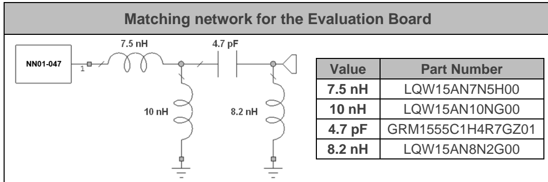
Figure 2 – Matching network implemented in the Evaluation Board.
