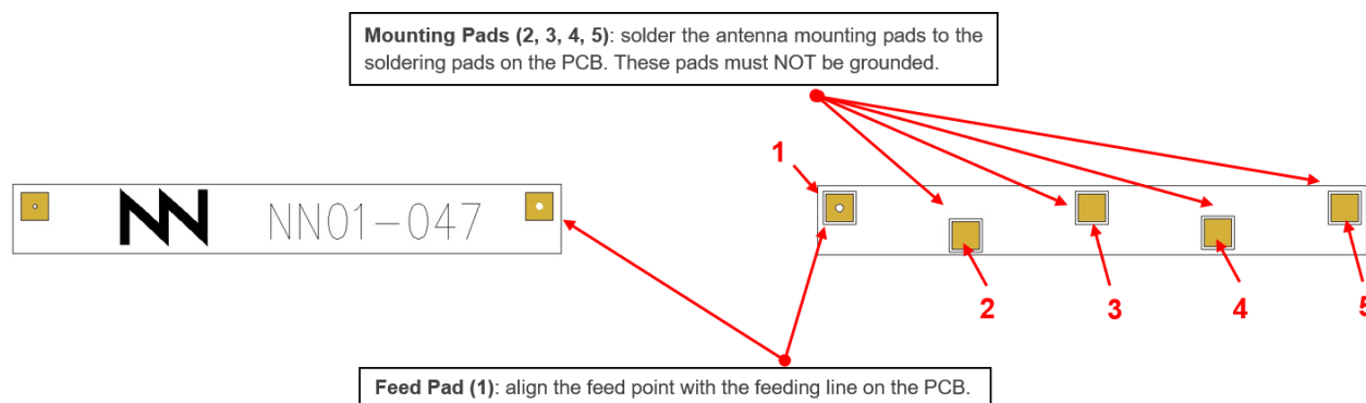
Figure 5 – Views of the TVNow™ Dual band (UHF+Lband) DVB-H antenna.
