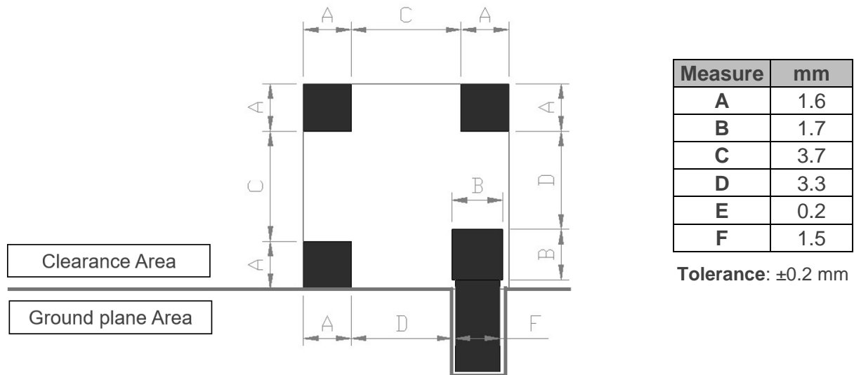
Figure 4 – Antenna Footprint Details.
