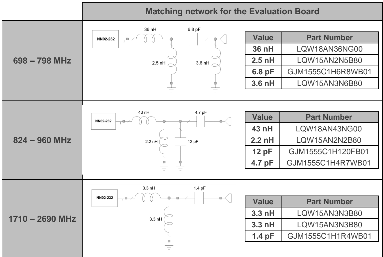
Figure 2 – Matching networks implemented in the Evaluation Board 3 ports (Figure 1).
