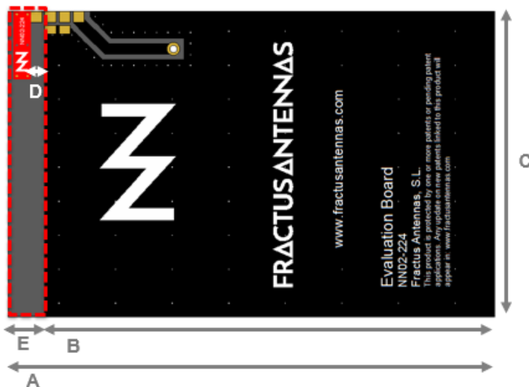
Figure 4 – EB_NN02-224-CR80-2,4-5 in CR80 standard format. Evaluation Board providing operation from 2.4 GHz to 2.5 GHz and from 4.9 GHz to 5.875 GHz.
