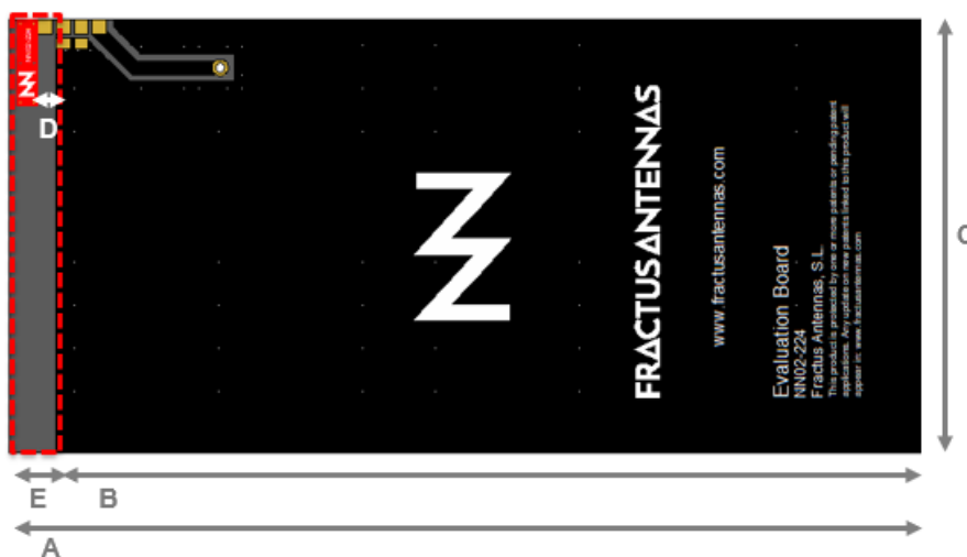
Figure 1 – EB_NN02-224-2,4-5. Evaluation Board providing operation from 2.4 GHz to 2.5 GHz and from 4.9 GHz to 5.875 GHz.
