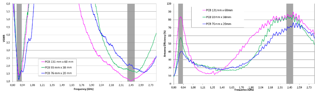
Figure 2 – VSWR and Total Efficiency for the 863 – 928 MHz and 2400 – 2500MHz from the evaluation board (Figure 1).
