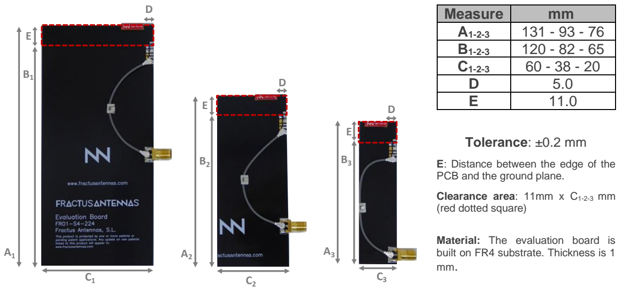
Figure 1 – Evaluation Board with different size dimensions providing operation from 863 MHz to 928 MHz and from 2400 MHz to 2500 MHz.
