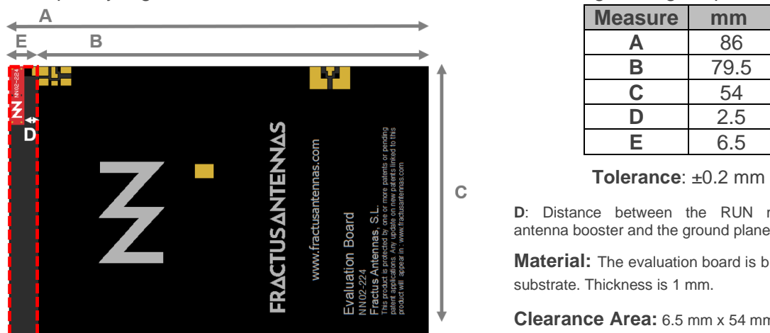
Figure 4 – EB_NN02-224-CR80-2400 in CR80 standard format. Evaluation Board providing operation from 2.4 GHz to 2.5 GHz.
