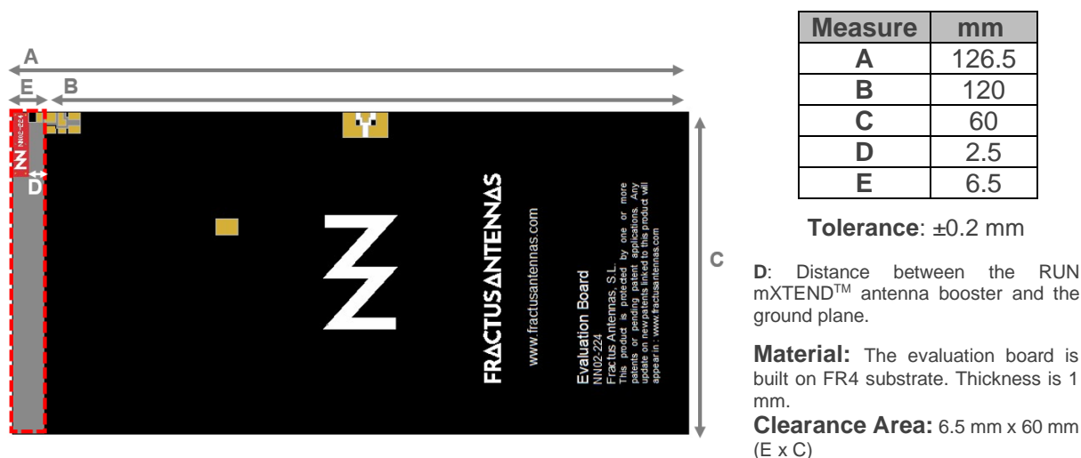
Figure 1 – EB_NN02-224-2400. Evaluation Board providing operation from 2.4 GHz to 2.5 GHz.
