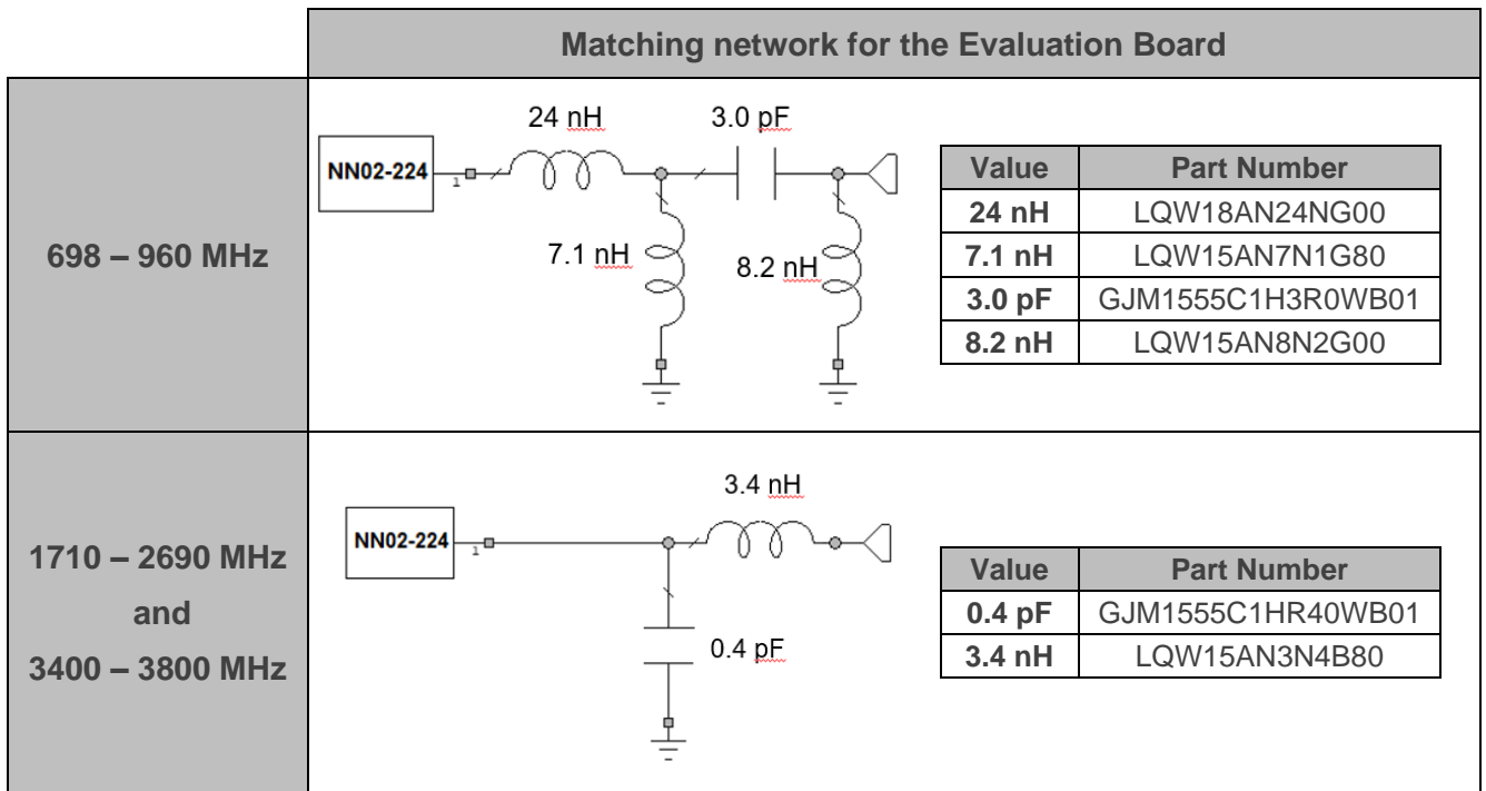
Figure 2 – Matching networks implemented in the Evaluation Board 2 ports (Figure 1).
