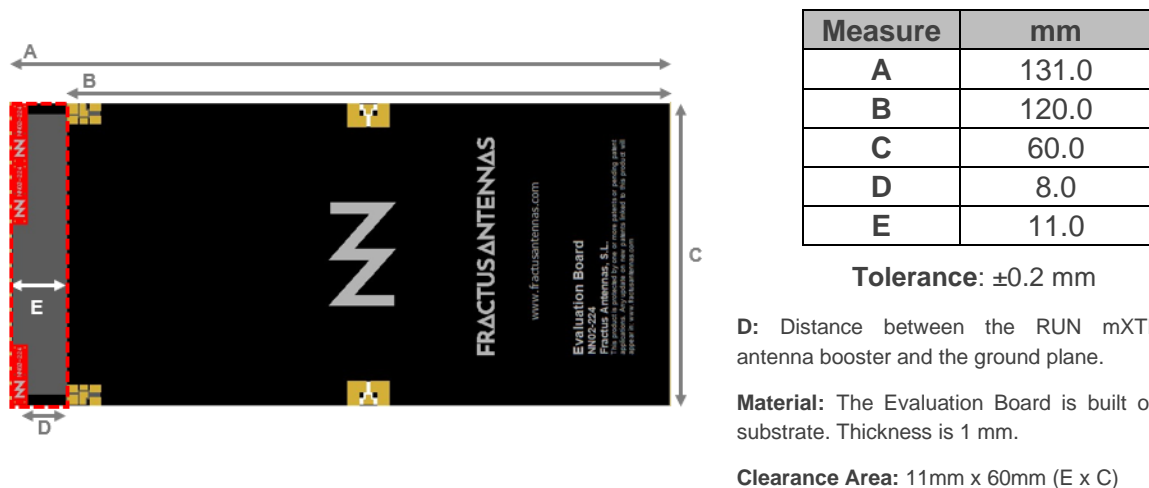
Figure 1 – EB_NN02-224-UFL3R-2P. Evaluation Board providing operation in 3 frequency ranges, 698 MHz to 960 MHz, 1710 MHz to 2690MHz, and 3400 MHz to 3800 MHz.
