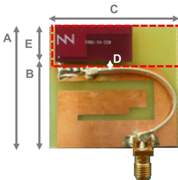
Figure 1 – NN02-220-SF1. Evaluation Board providing operation from 698MHz to 960MHz and from 1710MHz to 2690MHz.
