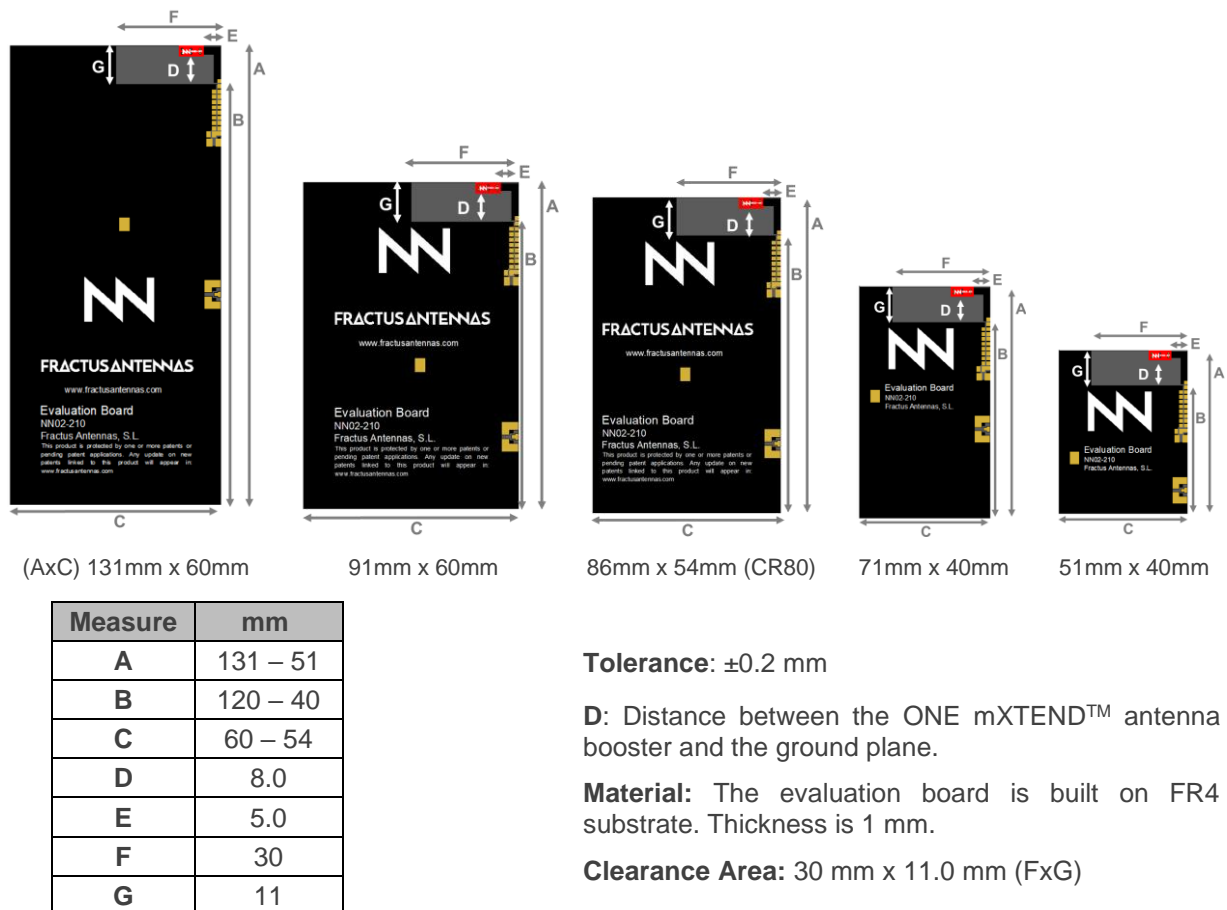
Figure 1 – Evaluation boards with different form factors and different EB sizes.
