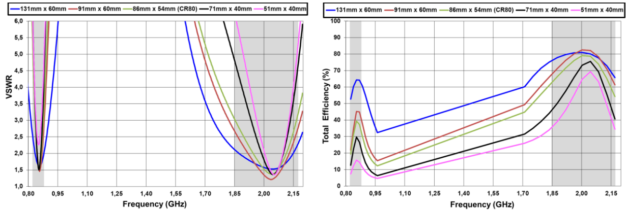
Figure 3 – VSWR and Total Efficiency for the 824 – 894 MHz frequency range and for the 1850 – 2170 MHz frequency range considering the different EB sizes (Figure 1).
