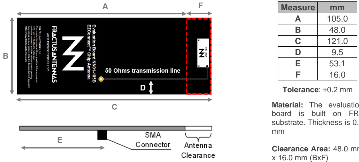
Figure1 – EB_NN01-105B. EZConnect™ Evaluation Board at 868 MHz.
