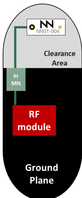
Example 3. With one NN01-004 antenna
