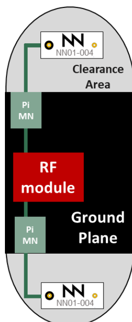
Example 4. MIMO with two N01-004 antennas
