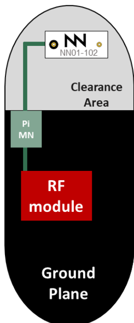
Example 1. With one NN01-102 antenna
