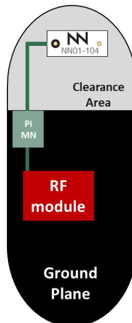
Example 2. With one NN01-104 antenna
