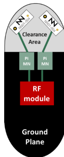
Example 4. MIMO with two NN01-004 antennas
