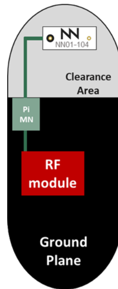
Example 2. With one NN01-104 antenna
