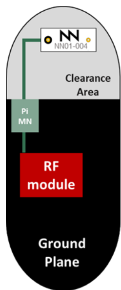
Example 3. With one NN01-004 antenna
