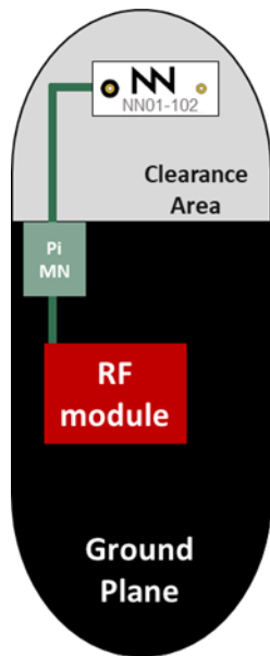
Example 1. With one NN01-102 antenna
